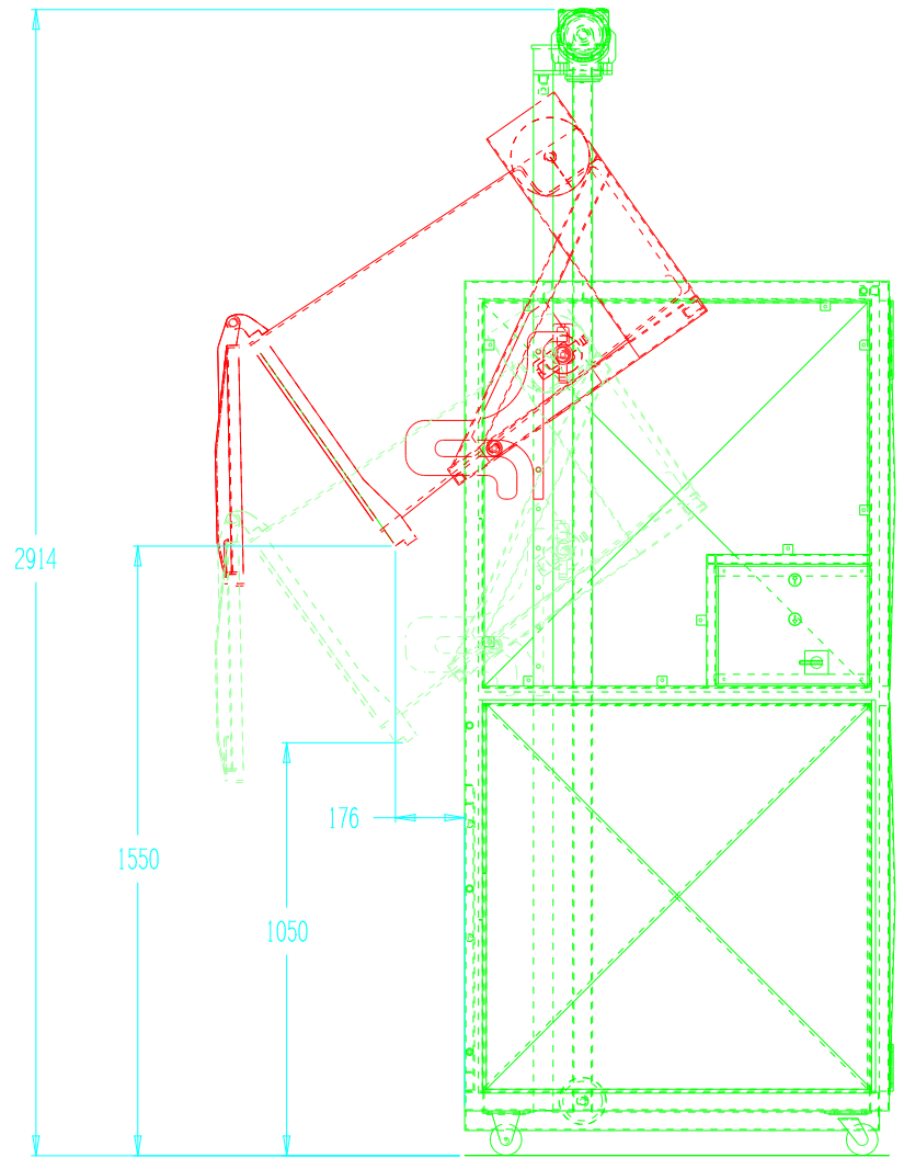
BASEWASTE 1000 120/240 LTR WHEELIE BIN TIPPER 1000mm TO 1500mm TIP HEIGHT (ADJUSTABLE IN 100mm INCREMENTS)
