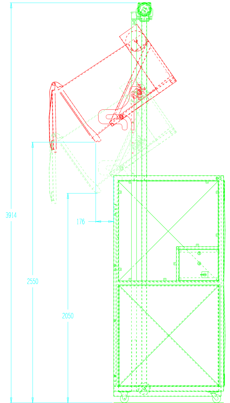
BASEWASTE 2000 120/240 LTR WHEELIE BIN TIPPER 2000mm TO 2500mm TIP HEIGHT (ADJUSTABLE IN 100mm INCREMENTS)
