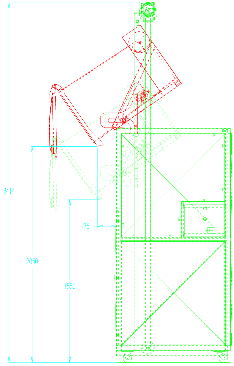
BASEWASTE 1500 120/240 LTR WHEELIE BIN TIPPER 1500mm TO 2000mm TIP HEIGHT (ADJUSTABLE IN 100mm INCREMENTS)
