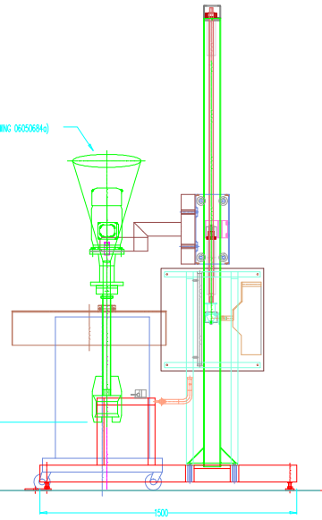
MIXER IN SMALLER VESSEL
