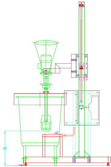
MIXER IN LARGER VESSEL
