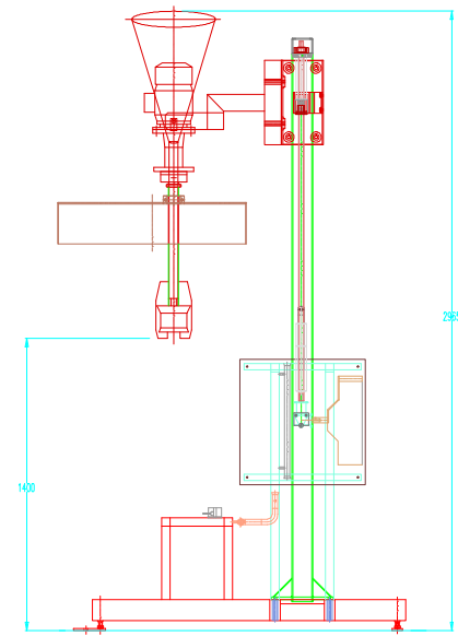
MIXER IN FULL UP POSITION
